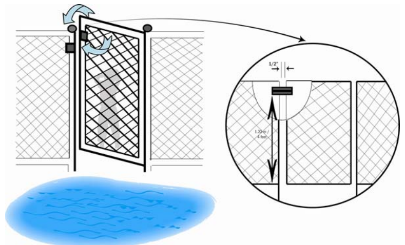
Figure 7: Self-closing and self-latching gate installation
